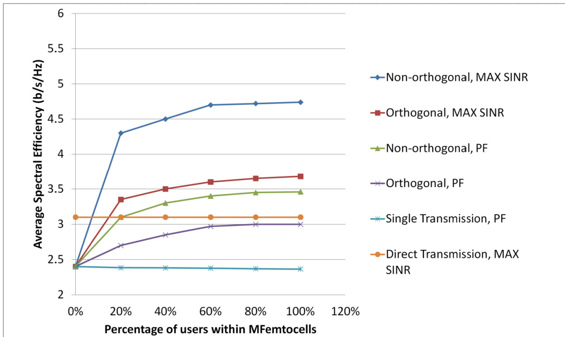
Fig. 7. Increase in percentage of users within the MFemtocells leads to more spectral efficiency in the case of the MFemtocells instead of the traditional direct scheme.
