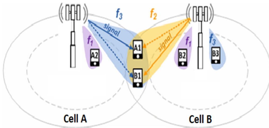
Fig. 3. Frequency resources for A1 and B1 at cell-edge are different because of ICIC method, causing no interference between them. While the same frequency is allocated to a less power consuming User Equipment (UE) because Cell A is already using that frequency for a UE at the cell-edge.
