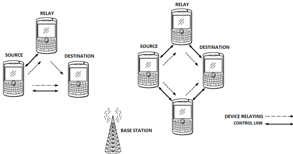
Fig. 12. Illustration of D2D communication with DC-DR.
