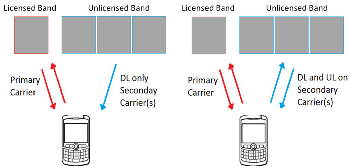
Fig. 1. (a) Primary carrier configured as both UL and DL, while Secondary carrier configured as DL only. (b) Primary carrier and Secondary carrier both configured as UL and DL.
